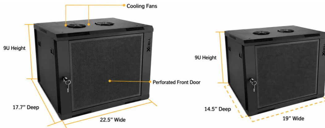
Product Dimensions
